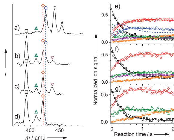
Figure 1. Temperature-dependent product-ion mass distributions and kinetics of the reaction of Au 2 + with CH 4 . Mass spectra have been recorded after trapping Au 2 + for 0.1 s inside the ion trap at a) 200 K, b) 250 K, c) 270 K, and d) 300 K. The corresponding reaction kinetics were obtained at e) 250 K (0.04 Pa CH 4 ; 1.02 Pa He), f) 270 K (0.04 Pa CH 4 ; 1.0 Pa He), and g) 300 K (0.08 Pa CH 4 ; 0.96 Pa He). See text for details. □ Au 2 + ; △ Au 2 (CH 4 ) + ; ◇ Au 2 (C 2 H 4 ) + ; ○ Au 2 (CH 4 ) 2 + ; ▽ Au 2 (C 2 H 4 )(CH 4 ) + ; ☆ Au(C 2 H 4 )(CH 4 ) + ; + Au 2 (CH 4 ) 3 + ; * Au 2 (C 4 H 12 ) + .
